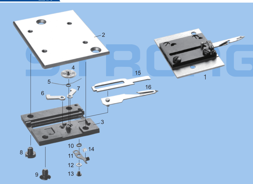
LZ-2290 剪线组件 ASSEMBLY FOR LZ-2290
