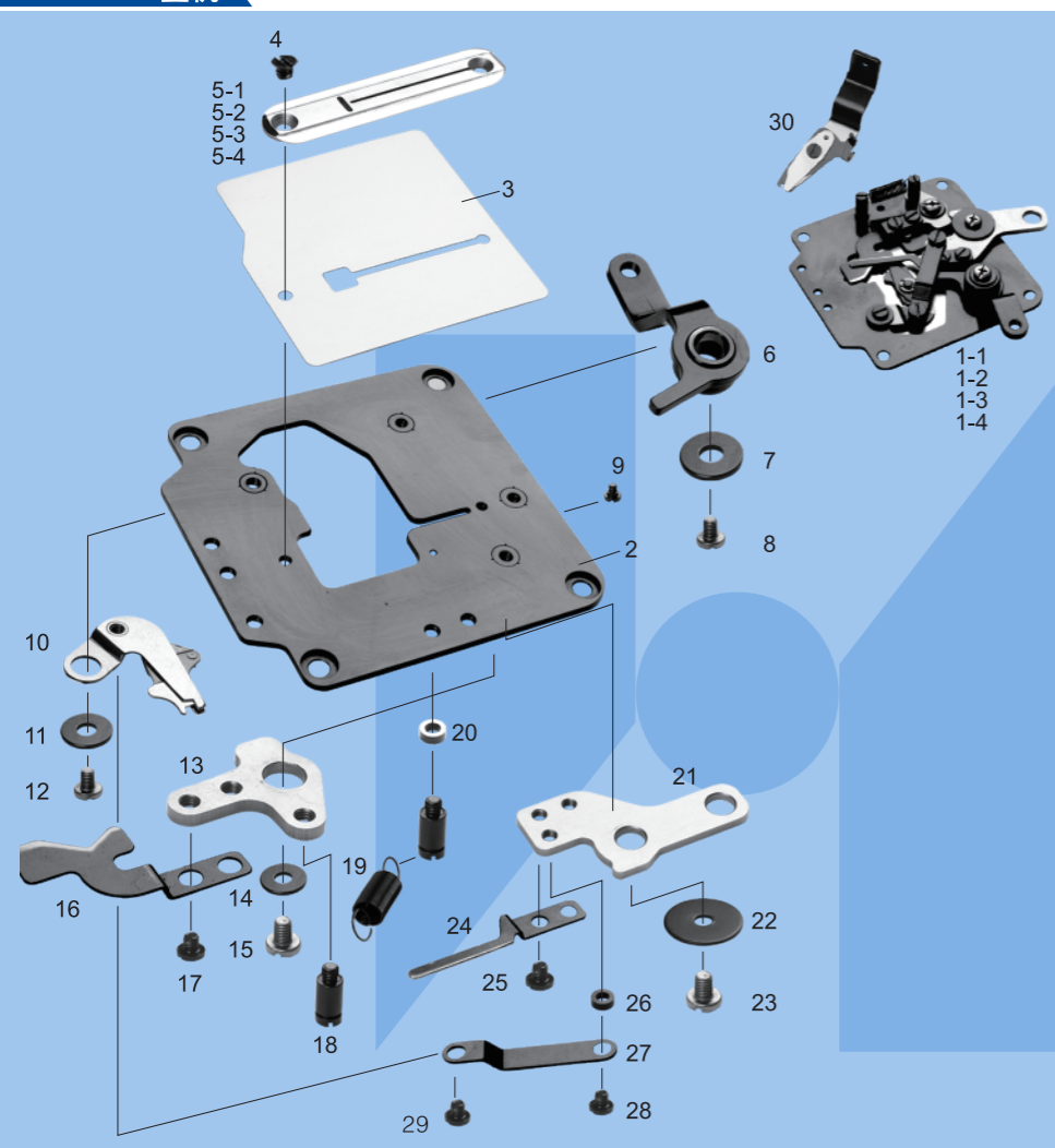
LBH-1790 剪线组 ASSEMBLY FOR LBH-1790
